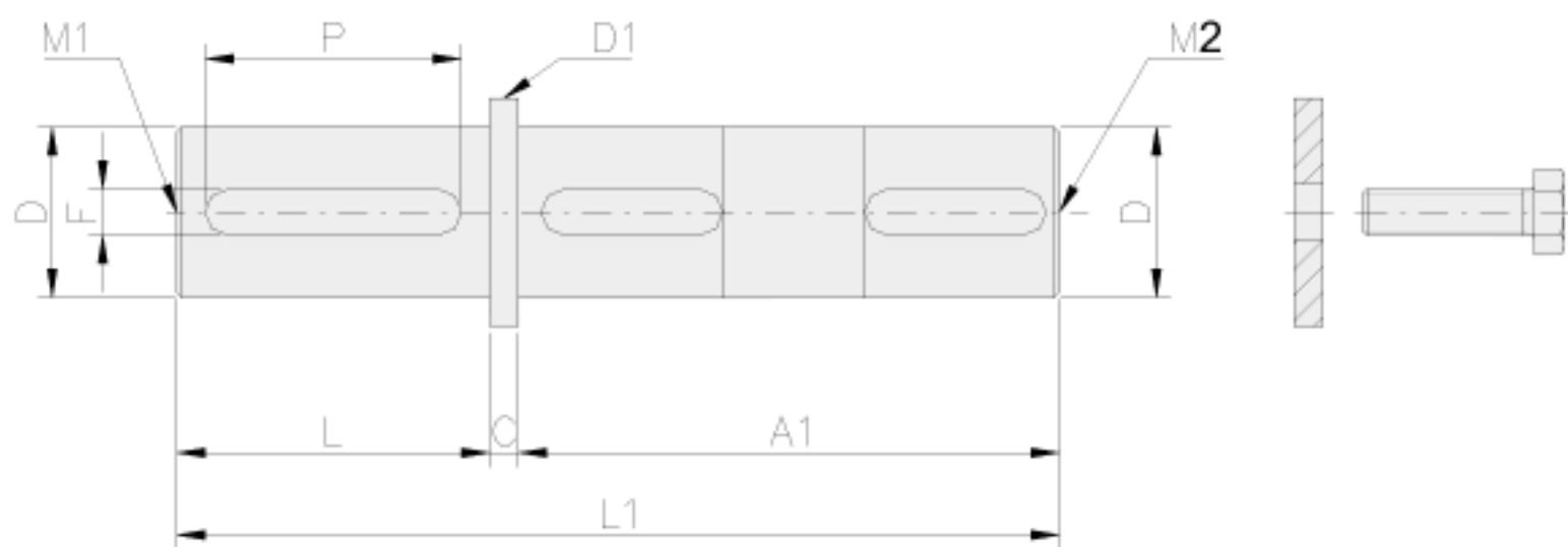
Output Shaft - single sided
