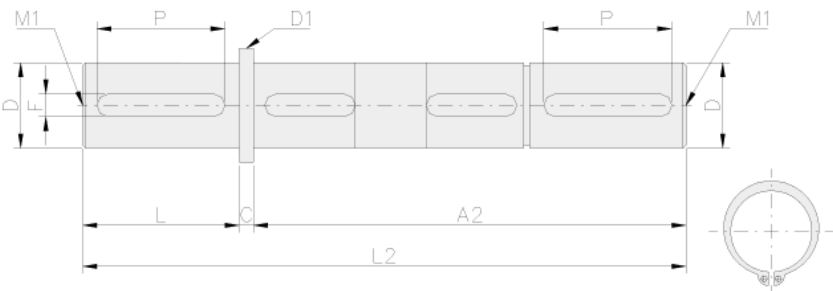
Output Shaft - double sided
